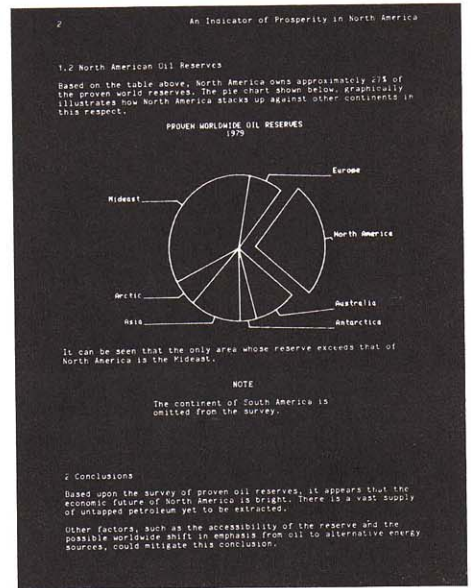
Document Preparation
