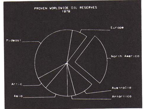
Easy Graphing
