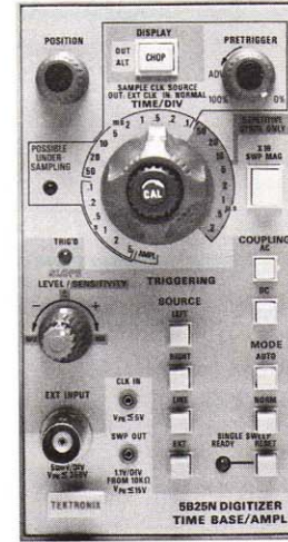
Digitizer Time Base/Amplifier
