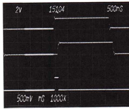
figure 2. The propagation delay time between the input of a delay line (upper trace) and the output of the delay line (middle trace) is measured digitally. Lower trace is 7D15 pseudo gate display. CRT readout displays the result of 151.0 ns.
