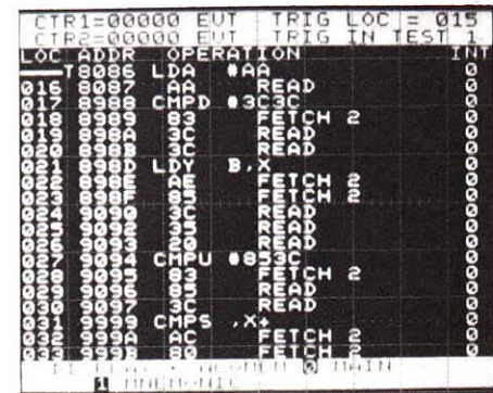
6809 Mnemonic Display
