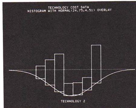
Statistics
