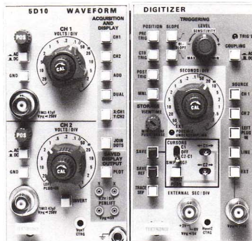
Waveform Digitizer
