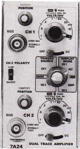
Dc to 400 MHz Dual Trace Amplifier
