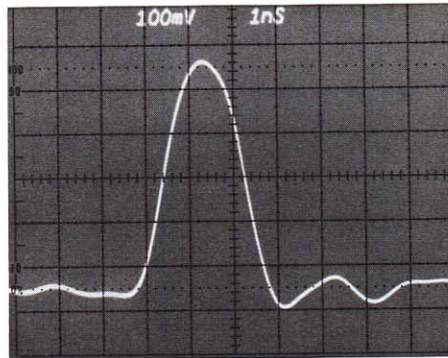
View of a single clocking pulse 0.8 ns rise and 2 ns pulse width.
