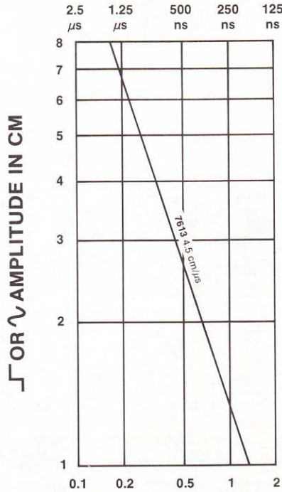
Graph showing the stored writing speed needed for a given sine wave or step rise time at a given amplitude.
