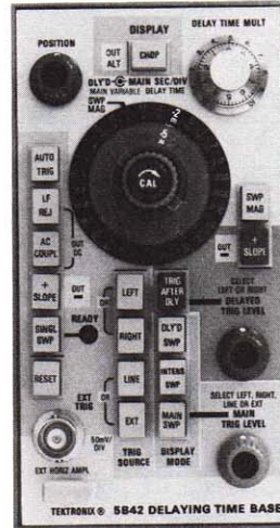
Delaying Time Base
