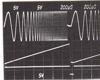
FG 507 in logarithmic sweep with sweep ramp and gate outputs.
