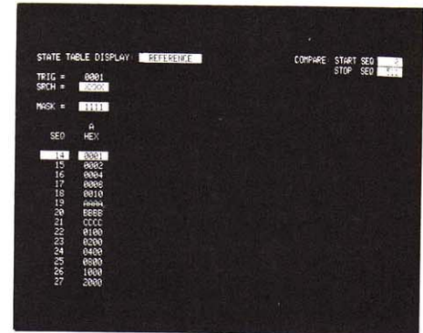
Figure 8. Reference Memory
