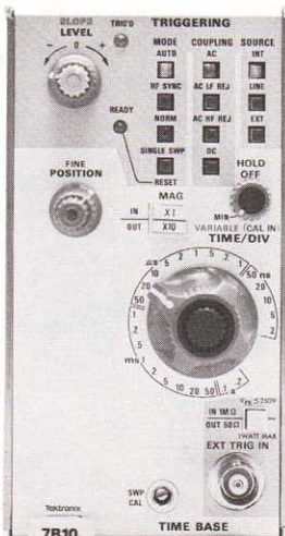
Delayed Time Base
