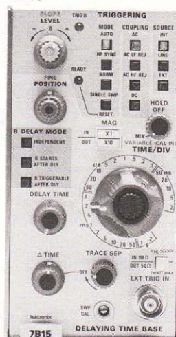
Δ Delaying Time Base
