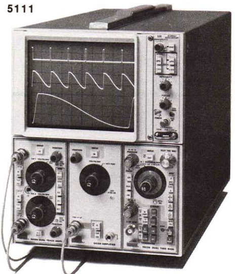
Single Bistable Beam Storage
