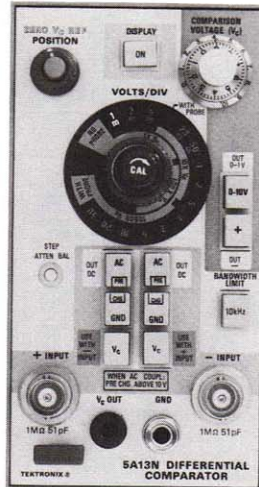
Differential Comparator
