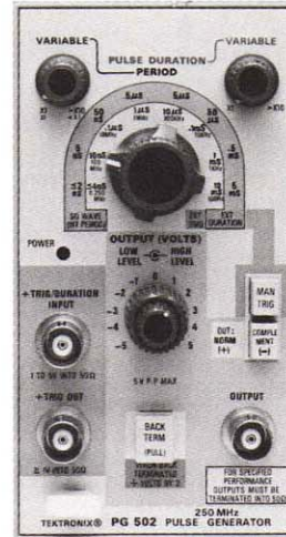
250 MHz Pulse Generator
