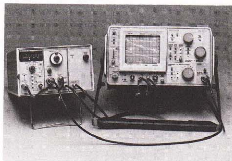
The 492 or 496 with TR503 Tracking Generator constitutes a calibrated swept frequency source covering 100 kHz to 1.8 GHz.
