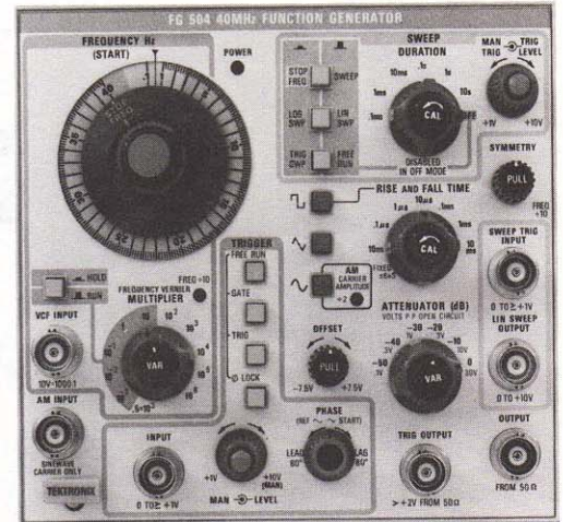
40 MHz Function Generator
