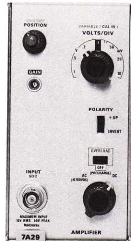
Dc to 1 GHz Amplifier
