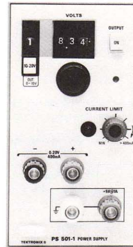
Power Supply
