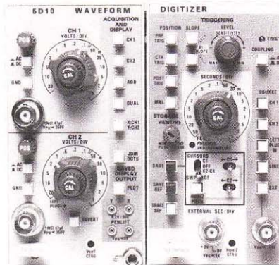
5D10 Waveform Digitizer
