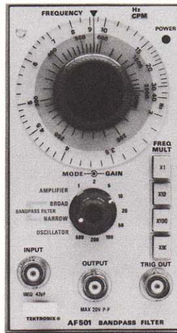
Bandpass Filter/Amplifier
