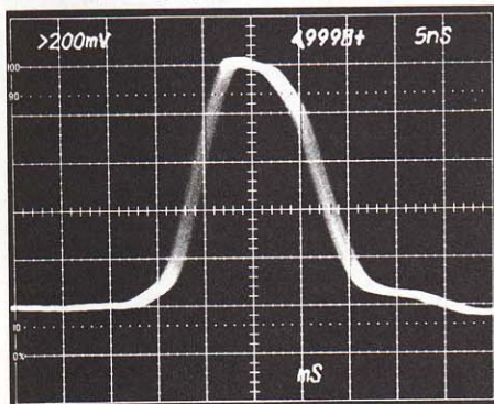
figure 1. Delay-by-time. A 0.2 \mu s time marker delayed 4.9998 ms by the 7D11 and displayed at 5 ns/div.
