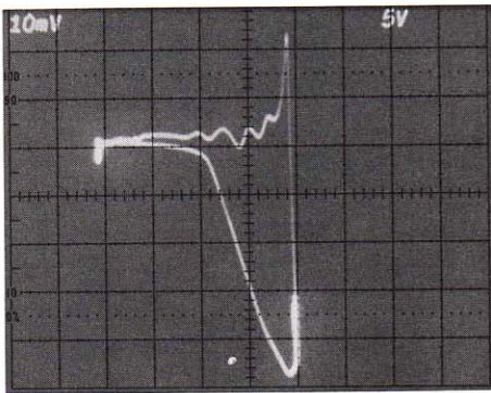
The transient load line of a fast switching transistor in a power supply prototype (switching time = 10 ns) is easily measured for compliance with safe operating area. (Horizontal = V; vertical = I).
