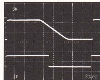
PG 508 output with fall times set 100 times longer than rise time.
