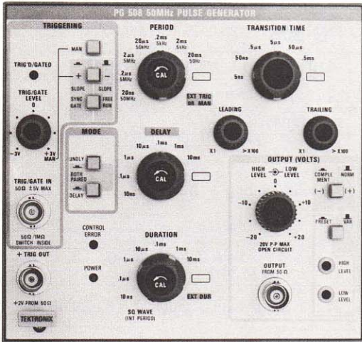
50 MHz Pulse Generator
