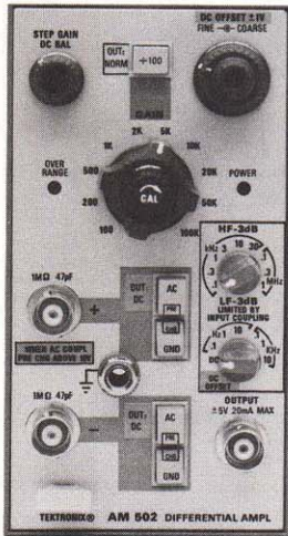
Differential Amplifier
