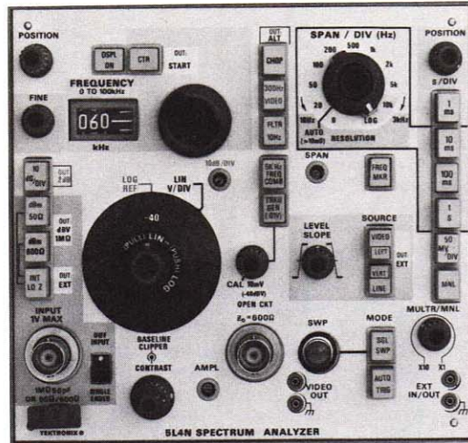
Spectrum Analyzer
