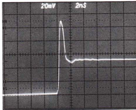
Circuit faults such as high frequency pulse overshoot and ringing can easily be observed with the 7104's 1 GHz bandwidth.
