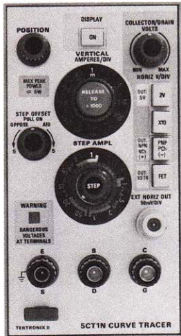
Curve Tracer
