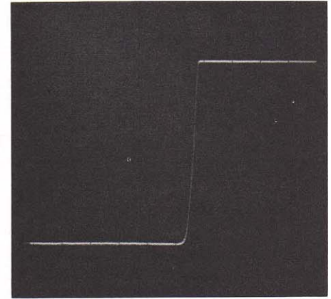
Film from the same pack was exposed to the same single-trace waveform and simultaneously to light from a Writing Speed Enhancer. The Enhancer light supplied the additional photons needed at the weak film development centers formed by the dim leading edge, to produce a visible image of the entire waveform.
