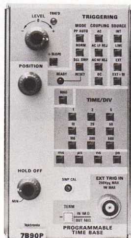
Programmable Time Base
