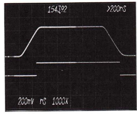
figure 3. Independent slope and level control allows the user to visually select precise points on the waveform where the counter starts and stops. CRT readout displays the result of 1543.9 ns.
