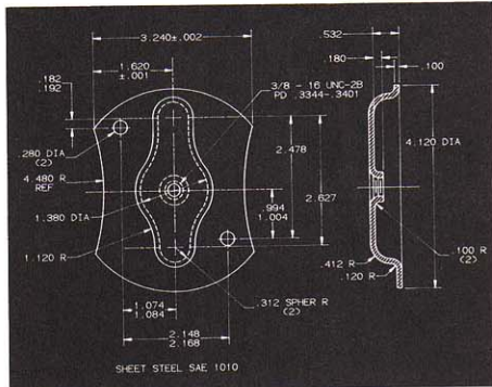
2-D Drafting
