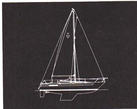
Picture Composition
