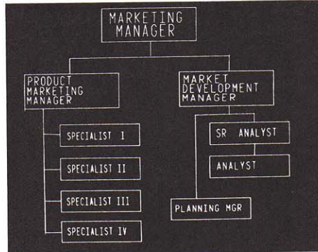
Picture Composition
