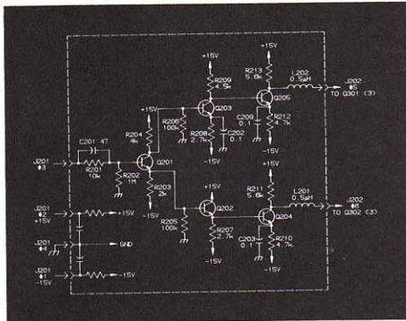
2-D Drafting
